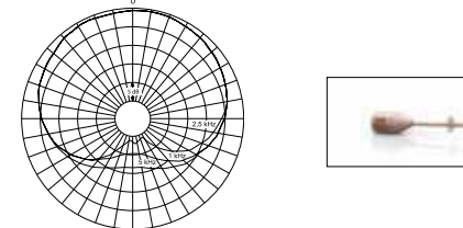
Polar Pattern (d:fine™ 4088 and d:fine™ 88)
